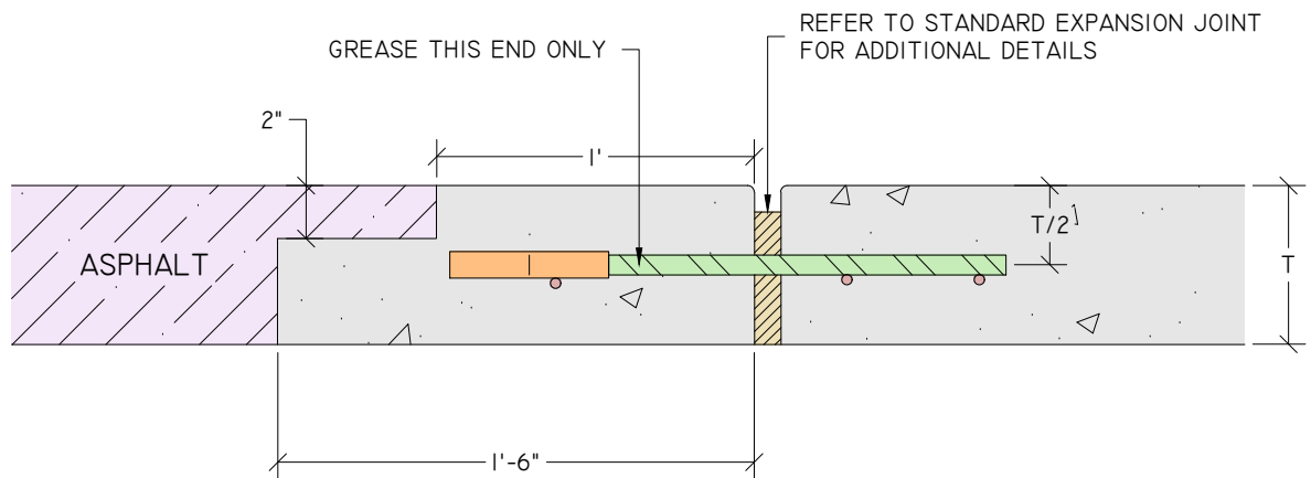
STANDARD CONCRETE HEADER FOR ASPHALT RETURN
