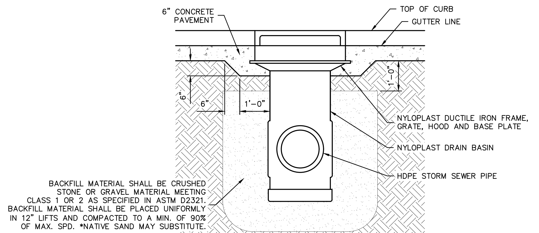
ALTERNATE PRIVATE CURB INLET DETAIL NOT TO SCALE
