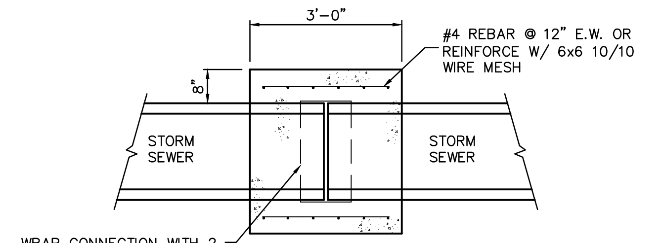
PIPE COLLAR DETAIL NOT TO SCALE
