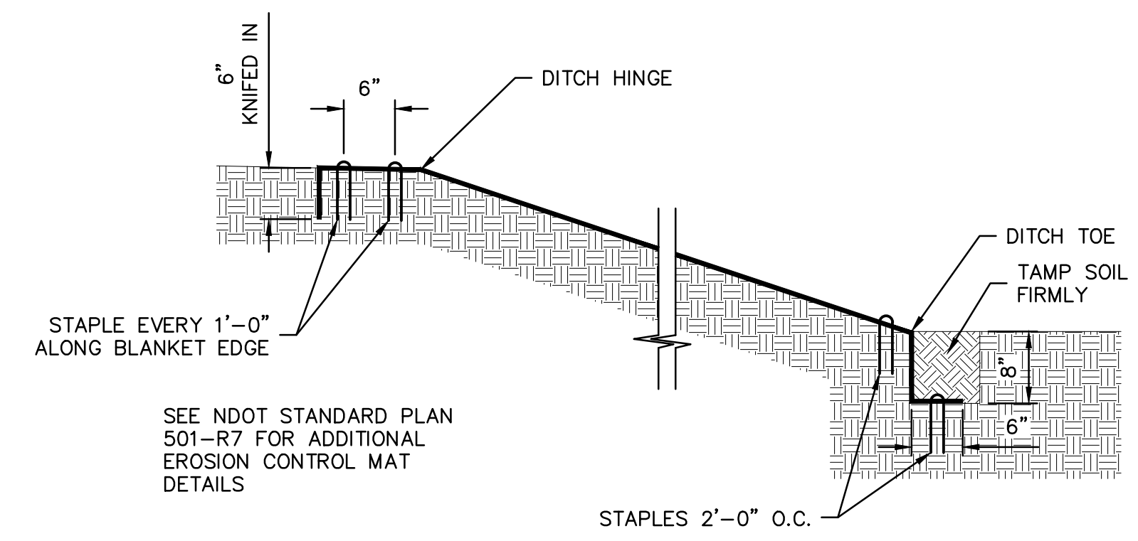
EROSION CONTROL MAT ANCHOR DETAIL NOT TO SCALE
