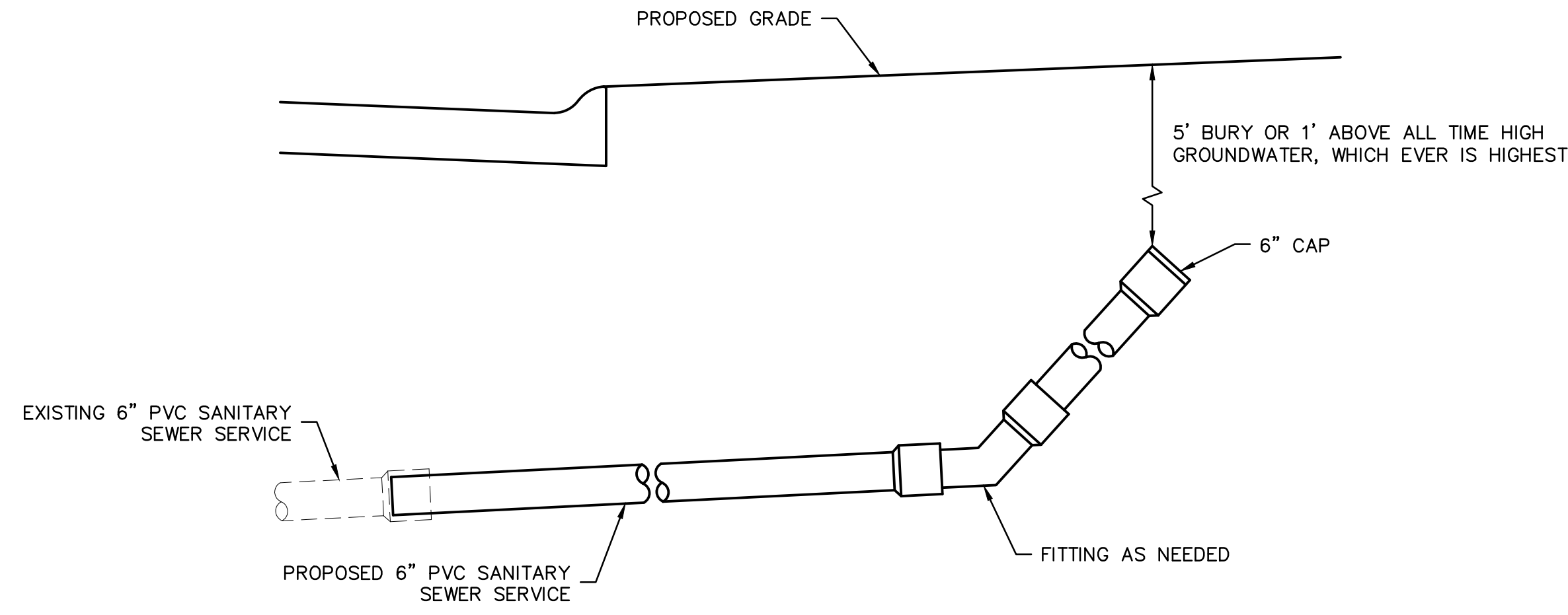
SANITARY SEWER SERVICE NOT TO SCALE
