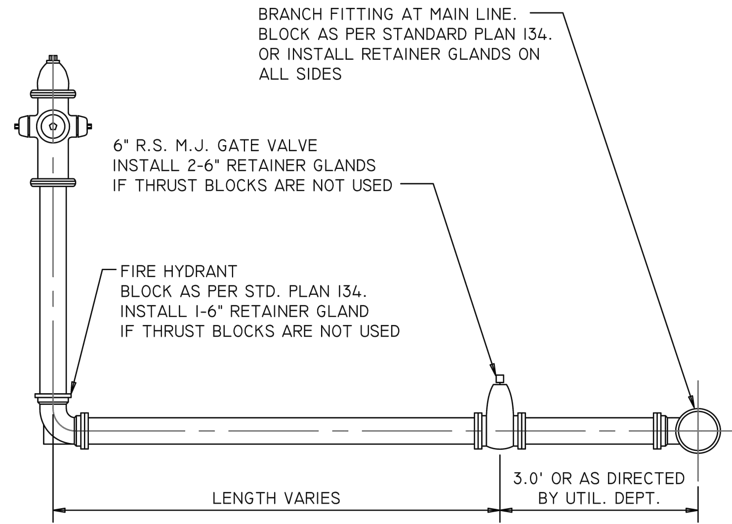
FIRE HYDRANT - TYPE 1 GRAND ISLAND STANDARD PLAN 140 NOT TO SCALE
