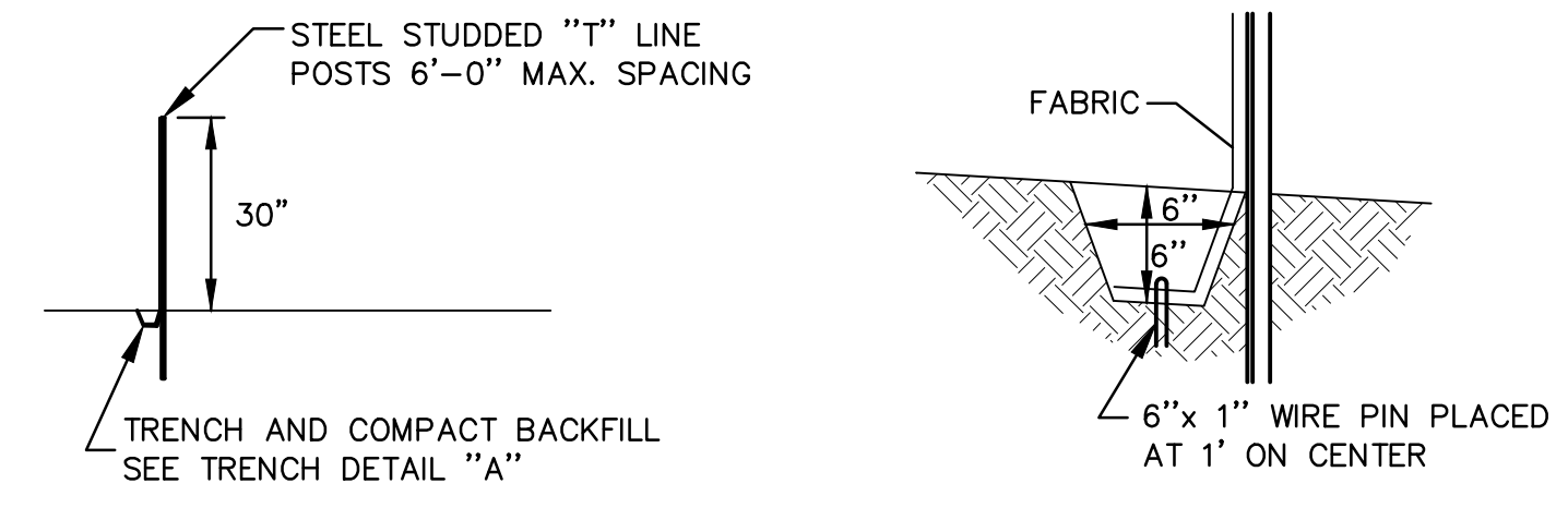
SILT FENCE DETAILS NOT TO SCALE
