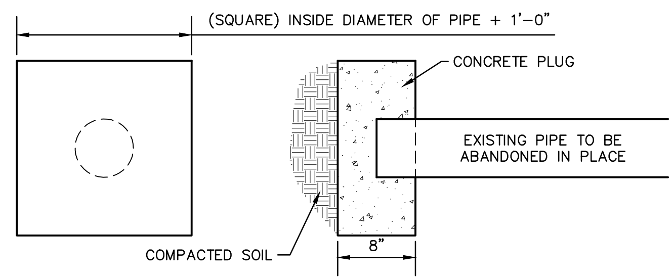
CONCRETE PLUG NOT TO SCALE
