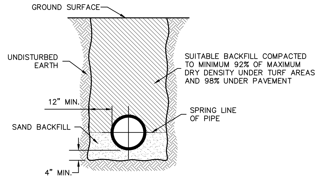
TRENCH BACKFILL NOT TO SCALE
