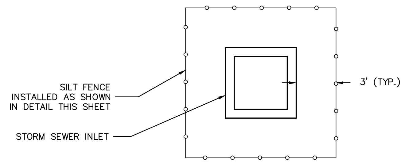
TEMPORARY INLET / MANHOLE PROTECTION NOT TO SCALE
