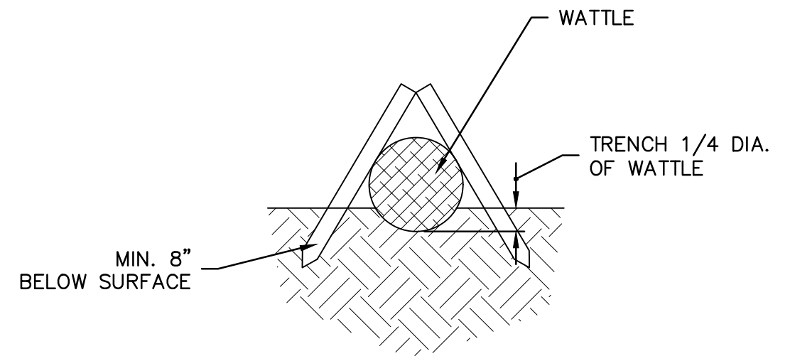
WATTLE DETAIL NOT TO SCALE
