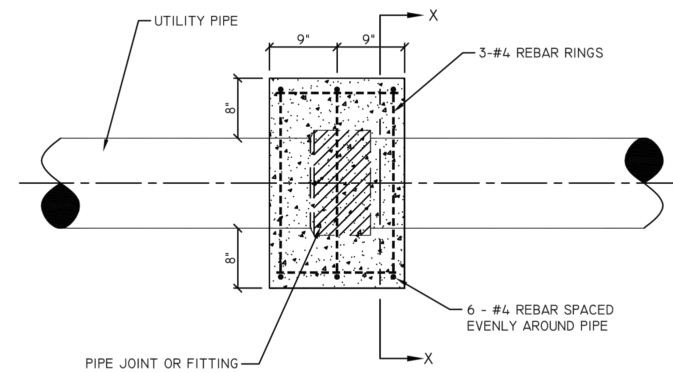
PLAN VIEW
