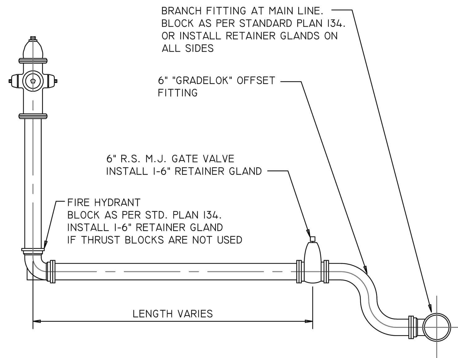
FIRE HYDRANT - TYPE 2 GRAND ISLAND STANDARD PLAN 140 NOT TO SCALE
