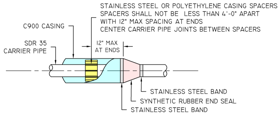
CASING DETAIL
