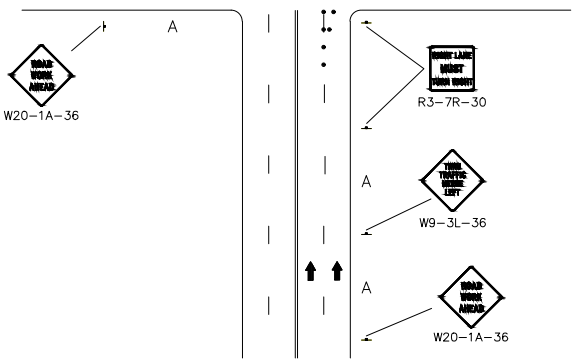
LANE CLOSED NEAR INTERSECTION (RIGHT LANE REMAINS OPEN)
