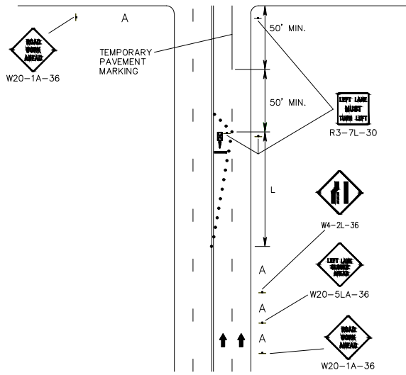
LANE CLOSED NEAR INTERSECTION (LEFT LANE CLOSURE FORMING A TURNBAY)
