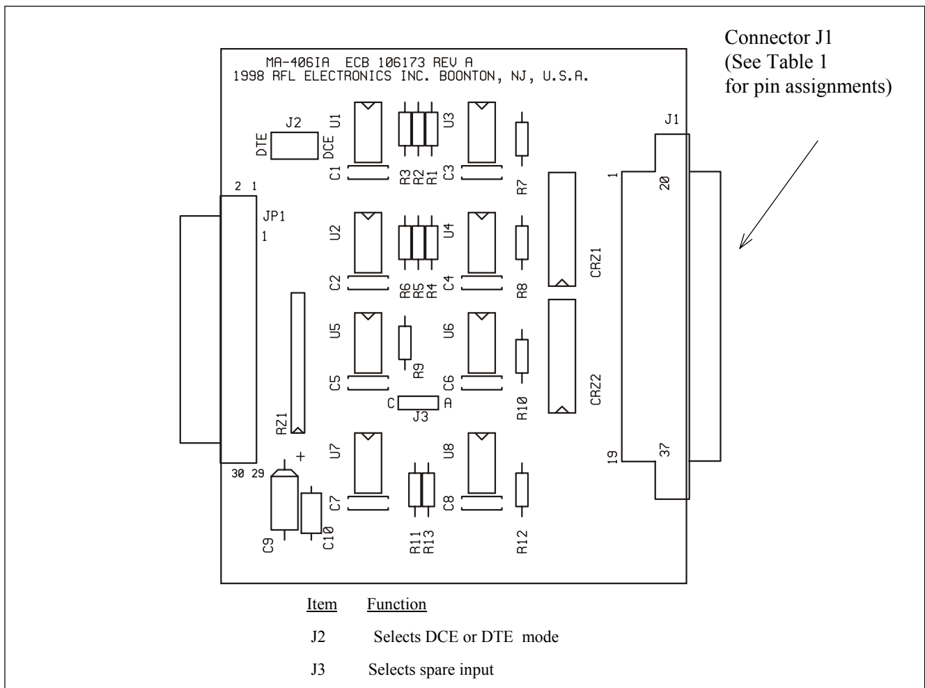
Figure 16- 1. Controls and indicators, MA-406IA Module Adapter
