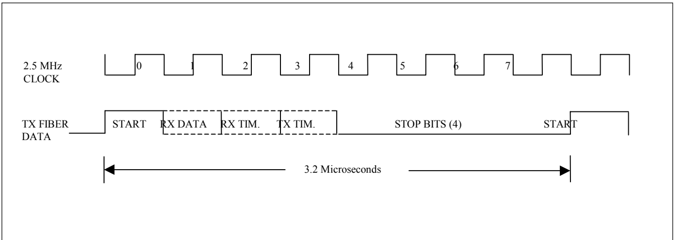
Figure 16- 8. Short Haul Fiber Timing Diagram
