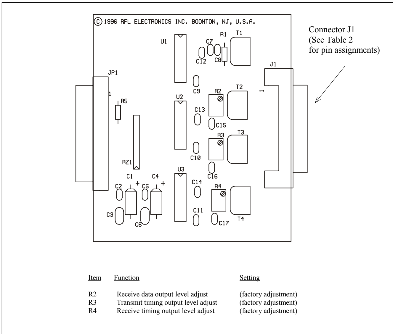
Figure 16- 2. Controls and indicators, MA-407I Module Adapter
