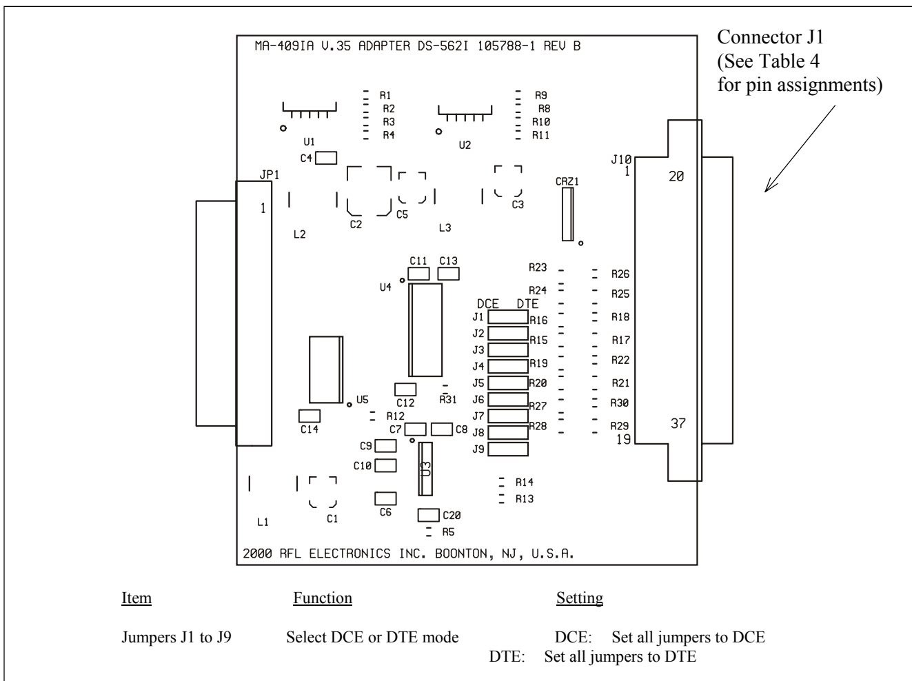
Figure 16- 4. Controls and indicators, MA-409IA Module Adapter
