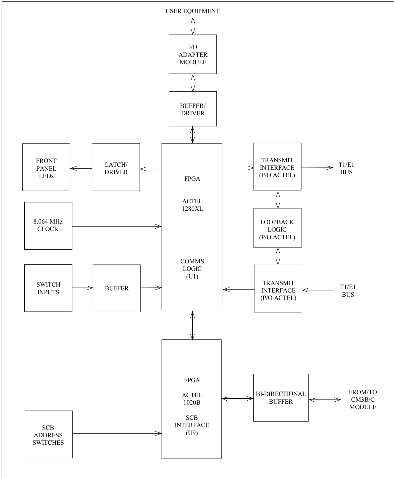
Figure 16- 9. RFL DS-562I Block diagram.
