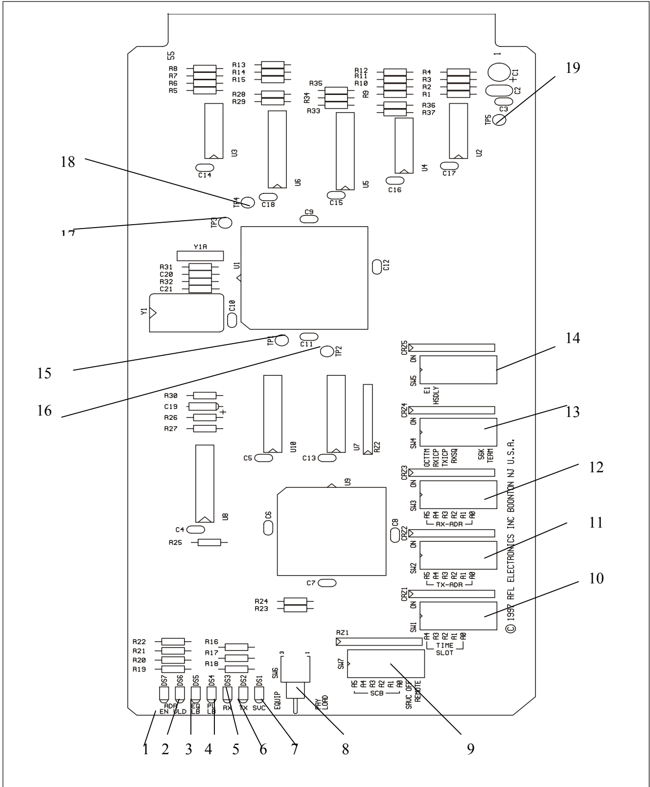
Figure 16- 6. Controls and indicators, RFL DS-5621 synchronous data module
