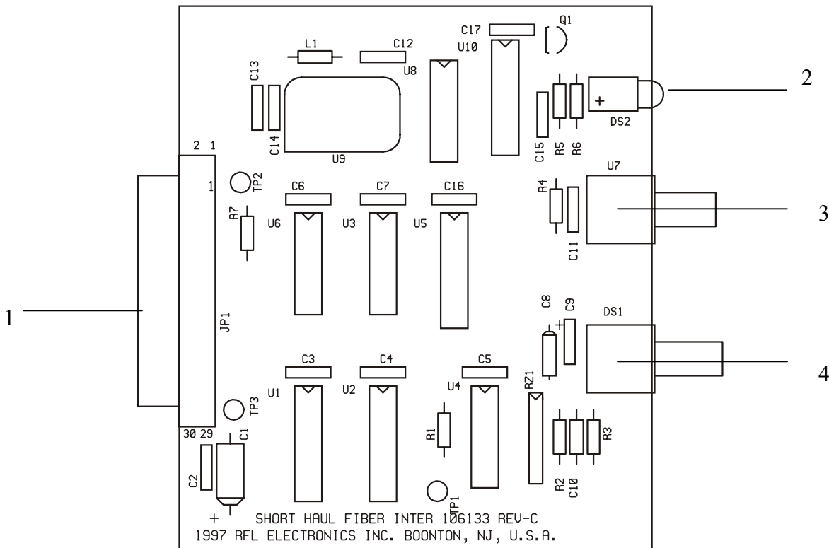
Figure 16- 7 Controls and indicators, MA-600 Module Adapter
