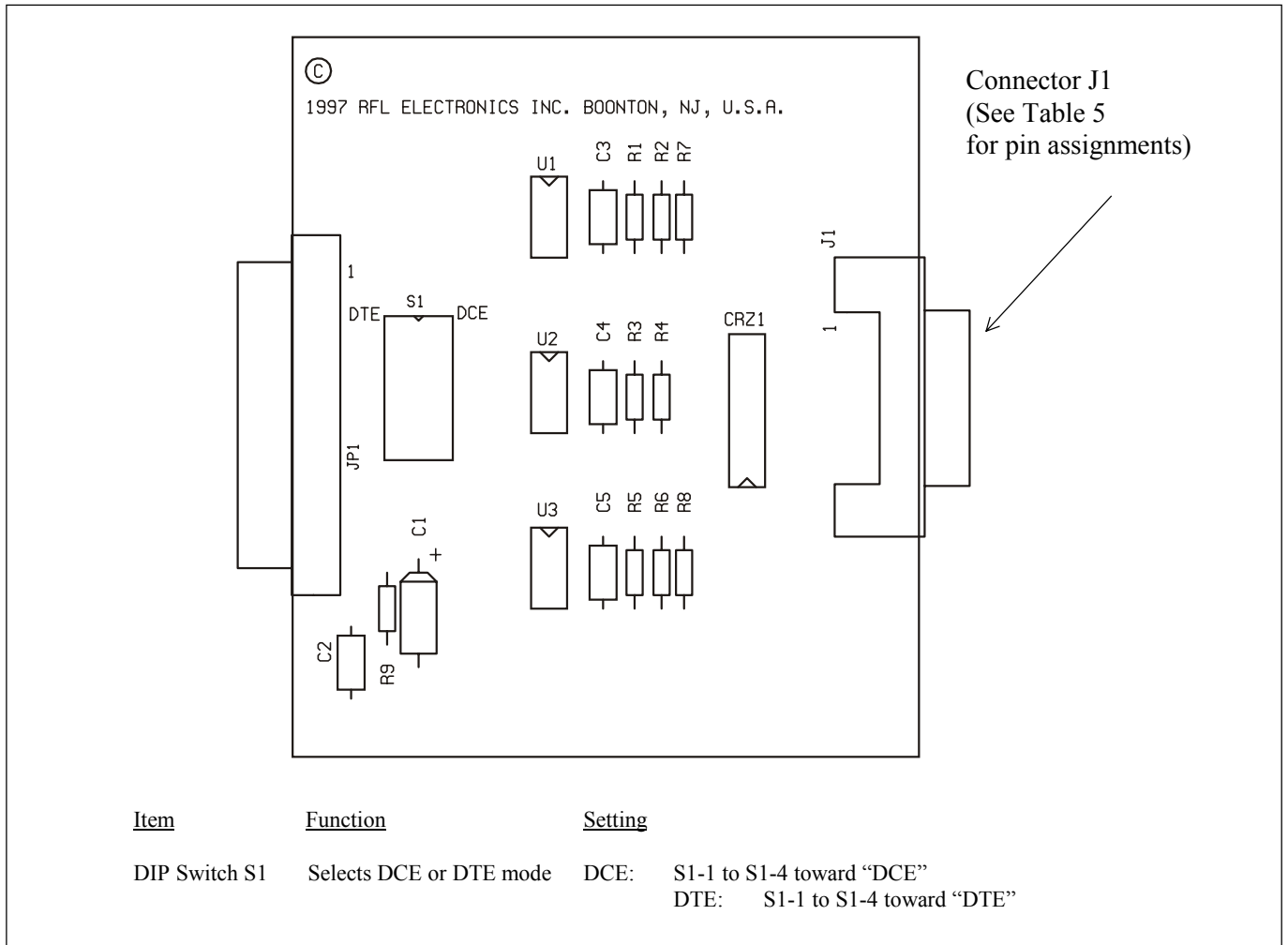
Figure 16- 5 Controls and Indicators, MA-410I Module adapter
