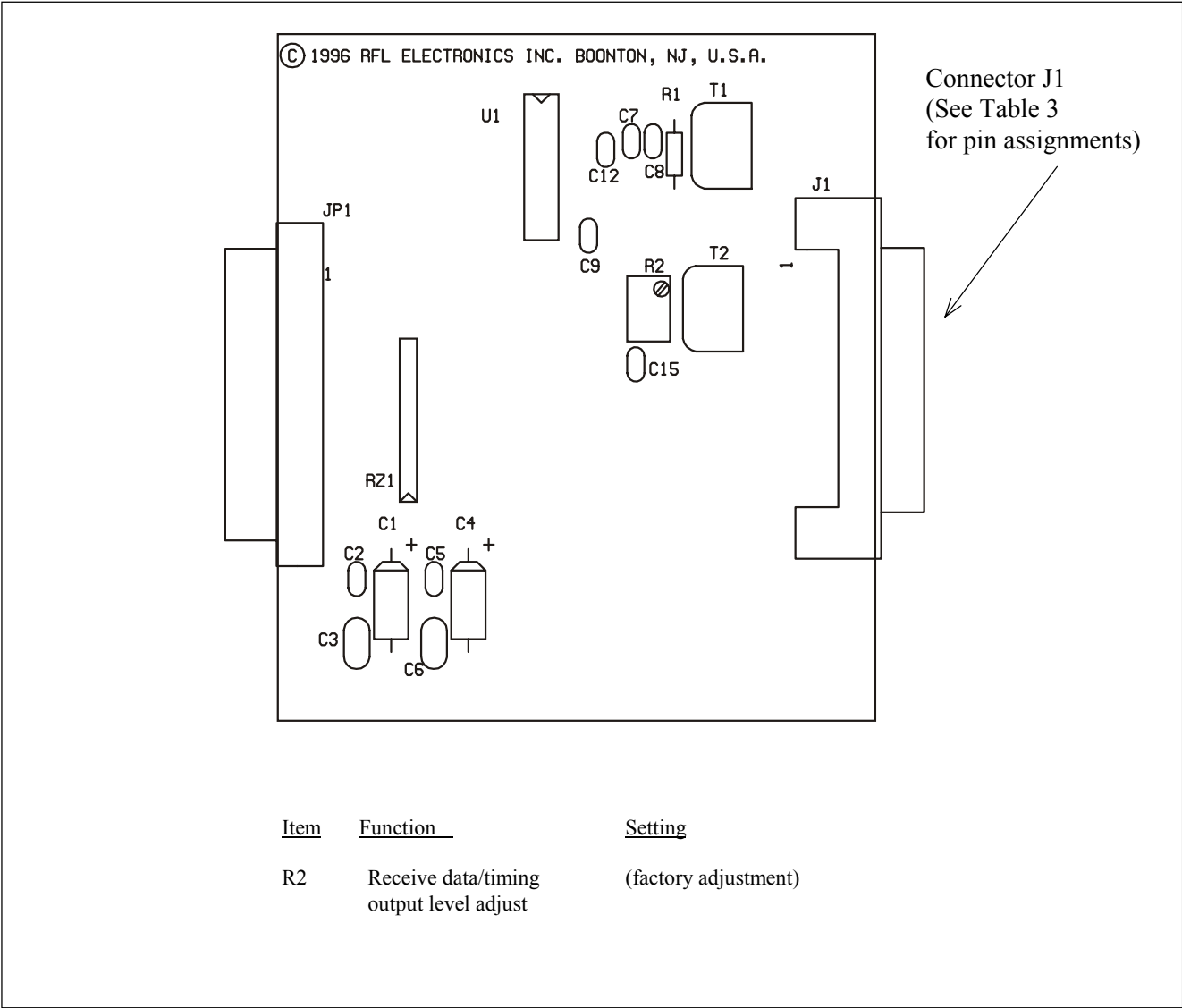
Figure 16- 3 Controls and indicators, MA-408I Module Adapter
