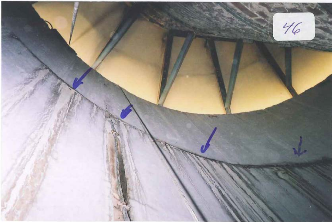
Photograph 46 thru 47 – NOT:E Rain hood and supports were found to be in good condition. The column appears to be leaking moisture through a cold pour joint.
