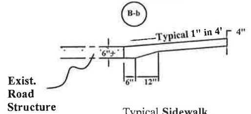
Typical Sidewalk Section
